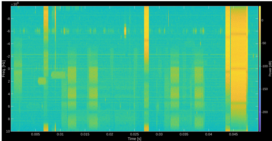
Figure 1: Example spectrogram.
